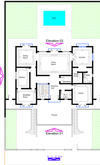
First Floor Plan A = 165,34 m 2
