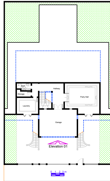
Lower Floor Plan A = 123,11 m 2
