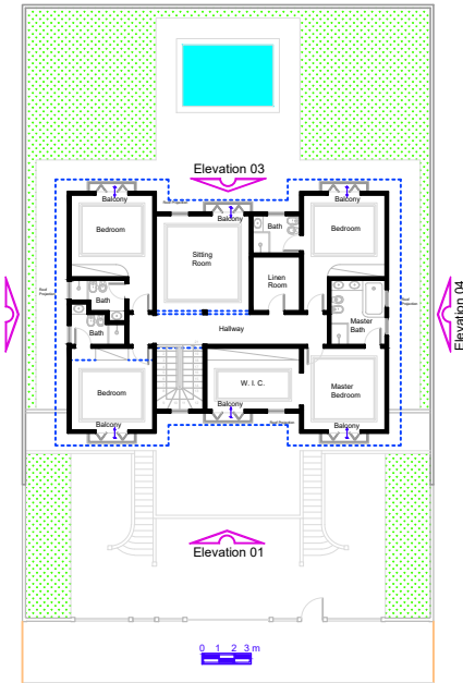
Second Floor Plan A = 169,48 m 2
