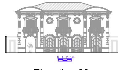
Elevation 03
